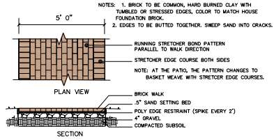
WALKWAY DETAILS
